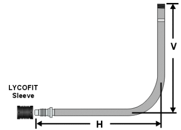
Field Assembled Transition Risers with LYCOFIT® Connection
