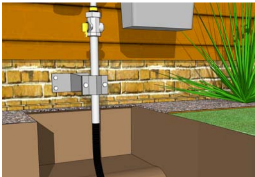
Lyall Riser Wall Brackets
